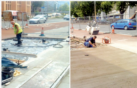
Removal of existing concrete road for services and reinstating following the completion of service installation.
